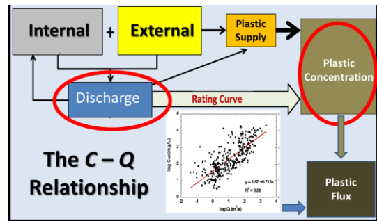
Watershed Factors
